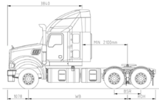
6x4 36" Stand-Up Sleeper Cab (914mm)
