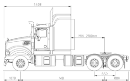
6x4 58" Sleeper Cab (1,473mm)
