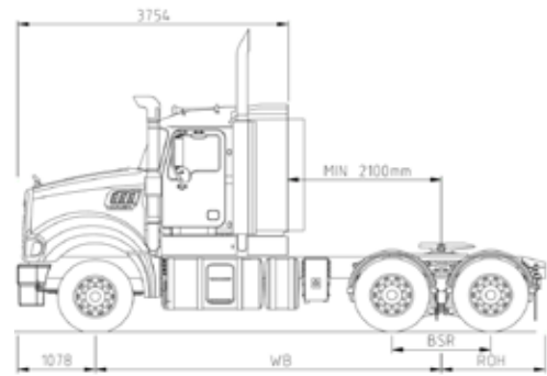
6x4 28" Super Cab (710mm)
