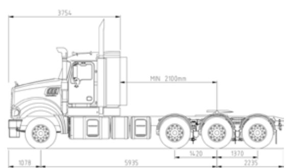
Mack Tri-Drive
