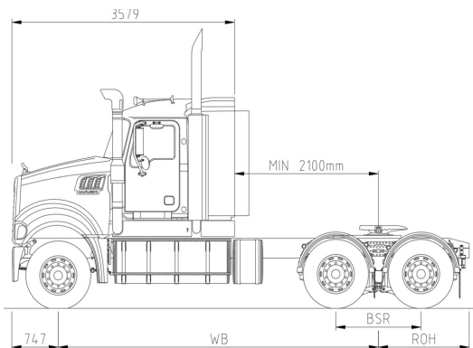
6x4 28" Super Cab (710mm)
