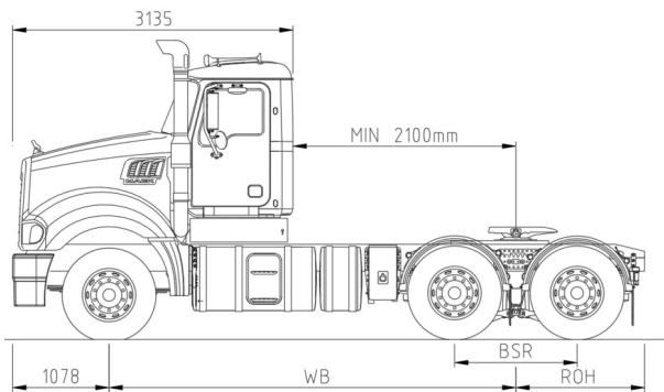
6x4 Day Cab Tractor
